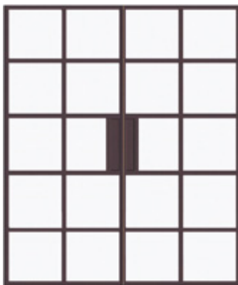
Sirius
