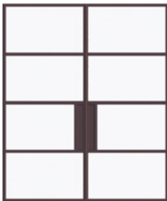
Bellatrix
